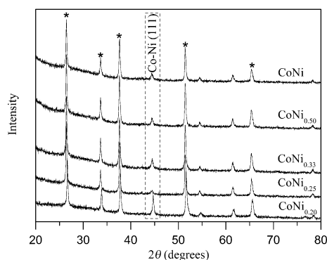
Figure 1. XRD patterns of binary Co-Ni alloy CEs. The diffraction peaks labeled with (*) were attributed to fluorine-doped tin oxide (FTO) conductive glass.
